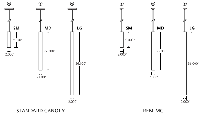
STANDARD CANOPY
