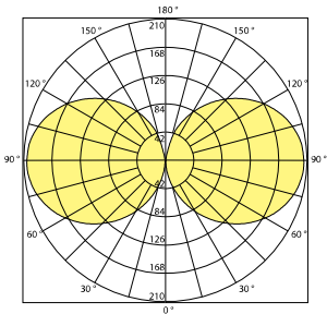
Delivered Lumens: 1090 lm Polar Candela Distribution
